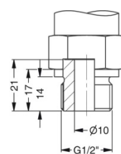
G1/2" open port DIN 3852 (up to 40 bar)
