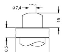
cable outlet with PVC cable (IP 67) 5
