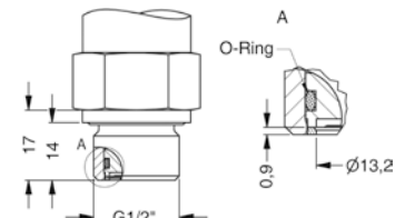
G1/2" DIN 3852 with flush sensor, P N ≤ 40 bar
