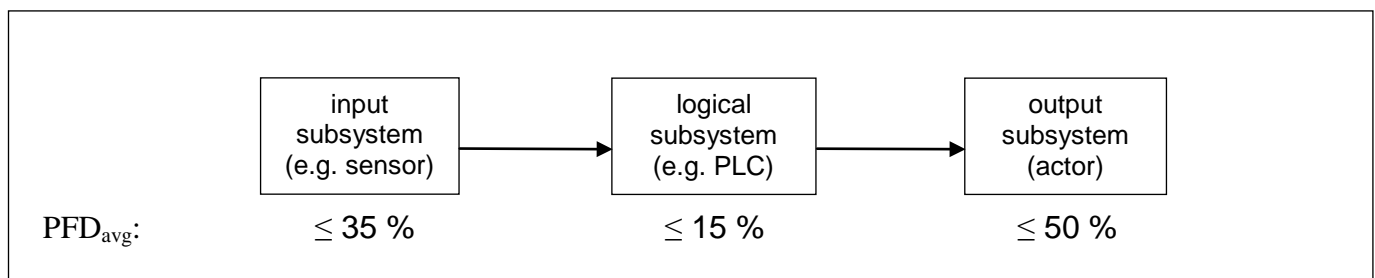
Fig. 2 usual fraction of PFD_{avg} to the subsystems
