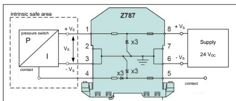
Fig. 3 Circuit diagram
