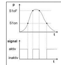
Fig. 3 compare mode
