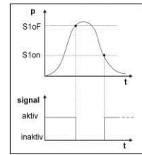
Fig. 6 hysteresis mode inverted
