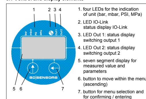
Fig. 3 Touch pad
