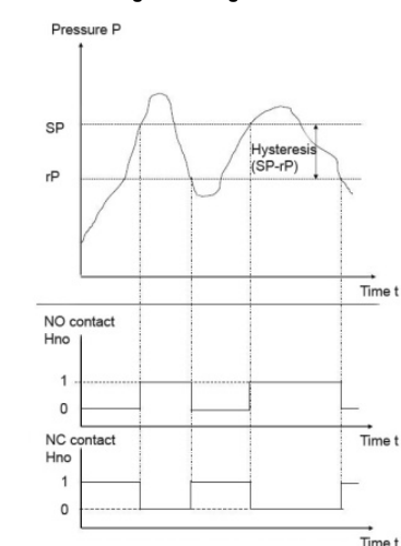
Fig. 4 Switching and resetting behaviour for hysteresis function in pressure-time graph
