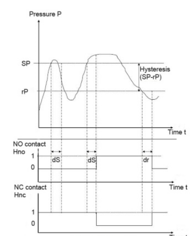
Fig. 5 Switching and resetting delay for hysteresis function in pressure-time graph
