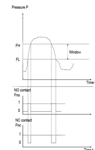
Fig. 6 Switching and resetting behaviour for window function in pressure-time graph
