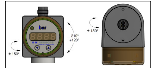
Fig. 2 display module (example with M12x1)
