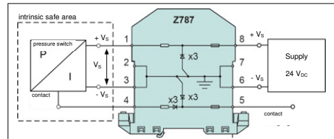
Fig. 4 circuit diagram
