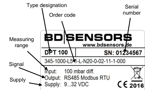
Fig. 1: Type plate
