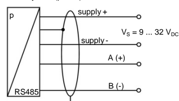
Fig. 2: Connection diagram
