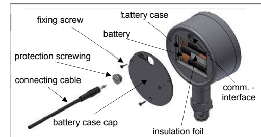
Fig. 3 Battery case and communication interface
