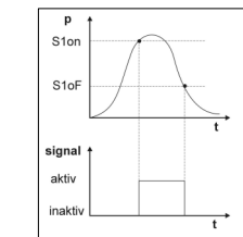
Fig. 7 hysteresis mode
