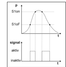
Fig. 6 compare mode
